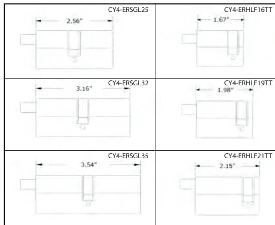
Full Euro Profile Cylinder
