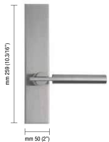
NERS Narrow Rectangular Escutcheon
